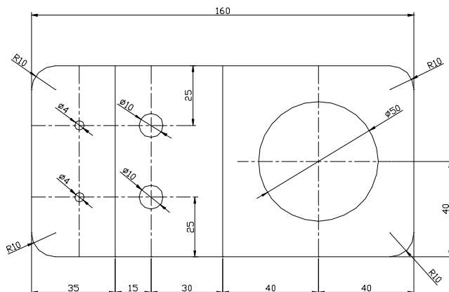
Working Drawing
